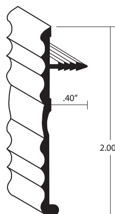
E-88 BD 2" Face
