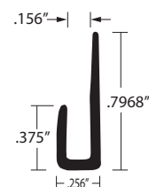
E-104 BA, EA 5/32" Material, Undrilled
