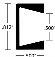
E-5165 EA 12' Shelf Face Cap For 3/4" Material, recommended use with dovetail cutter
