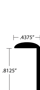
A-326 MF, BA Drilled & Undrilled
