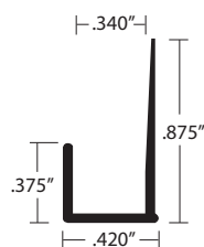
E-814 MF, EA 11/32" Material, Punched & Slotted
