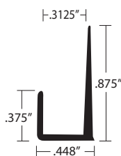
E-402 BA 5/16" Material, Undrilled
