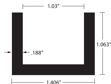
EAM-3195 MF Special Order
