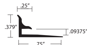
E-85 MFA 3/32" Material
