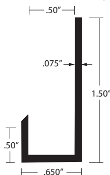
EAM-2627 MF For 1/2" Material, Undrilled
