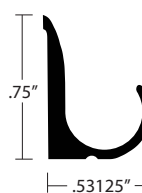
E-400 BD, EA Undrilled, Flat Back Tape Application
