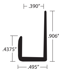
E-2465 BD 3/8" Material, Undrilled
