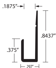
E-72 BA 3/16" Material, Undrilled
