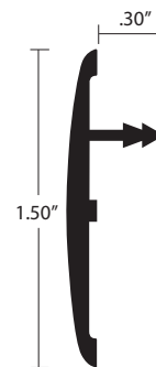
E-3898 MF, BD, EA
