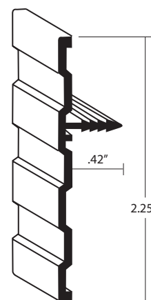
BST-214 BD 2-1/4" Face
