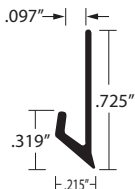
E-514 MF, EA 1/16" Material, Punched & Slotted
