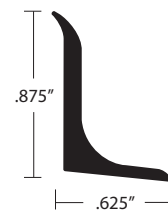
E-221 BD, EA Drilled & Undrilled (Drilled on long leg)
