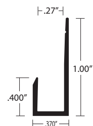
E-403 EA 1/4" Material, Undrilled
