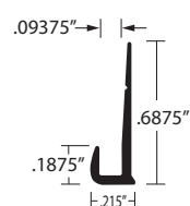
E-83 MFA 3/32" Material, Undrilled
