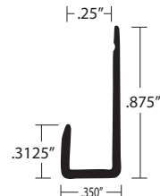
E-401 MF, BA, EA 1/4" Material, Punched & Slotted
