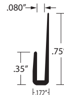
EAM-310 MF, BK, EA 1/16" Material, Undrilled
