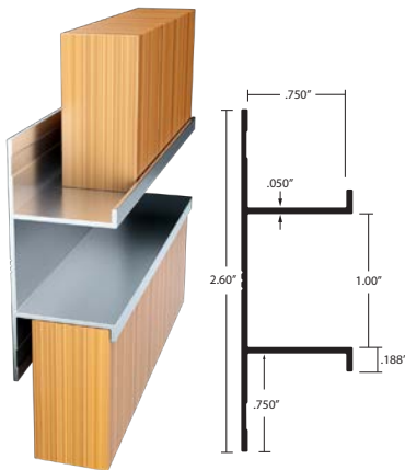
EMT-19 Flanged Channel 1" Reveal EMT-19075 - 3/4" Depth EA, MF
