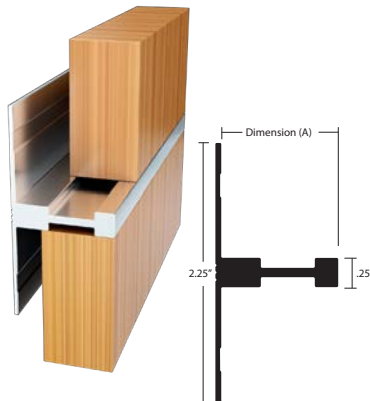
EMT-08 1/4" Accent EMT-08075 - 3/4" Depth (Dim A) EMT-82100 - 1" Depth (Dim A) EA, MF
