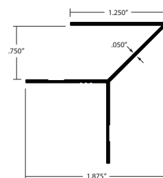
EMT-20 Extended Arrow Outside Corner EMT-20075 - 3/4" Depth EA, MF
