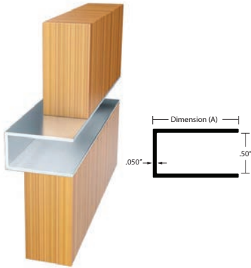
EMT-01 Millwork U Channel EMT-01075 - 3/4" Depth (Dim A) EMT-01100 - 1" Depth (Dim A) EA, MF
