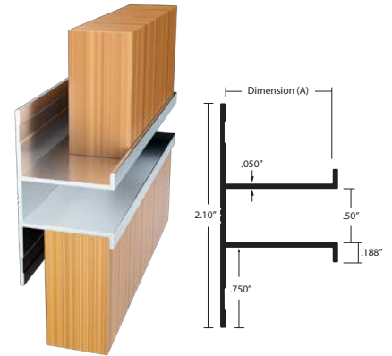
EMT-03 Flanged Channel 1/2" Reveal EMT-03075 - 3/4" Depth (Dim A) EMT-03100 - 1" Depth (Dim A) EA, MF
