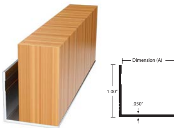
EMT-04 Millwork Angle EMT-04075 - 3/4" Depth (Dim A) EMT-04100 - 1" Depth (Dim A) EA, MF
