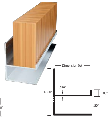
EMT-07 Flanged "F" 1/2" Reveal EMT-07075 - 3/4" Depth (Dim A) EMT-07100 - 1" Depth (Dim A) EA, MF
