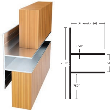
EMT-02 Channel 1/2" Reveal EMT-02075 - 3/4" Depth (Dim A) EMT-02100 - 1" Depth (Dim A) EA, MF
