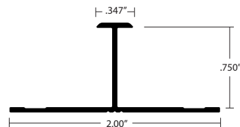
EMT-18 H-Mold EMT-18075 - 3/4" Depth (Dim A) EMT-18100 - 1" Depth (Dim A) EA, MF
