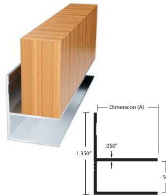
EMT-06 "F" 1/2" Reveal EMT-06075 - 3/4" Depth (Dim A) EMT-06100 - 1" Depth (Dim A) EA, MF
