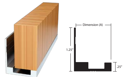
EMT-09 1/4" Termination Accent EMT-09075 - 3/4" Depth (Dim A) EMT-09100 - 1" Depth (Dim A) EA, MF
