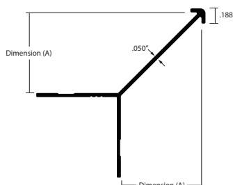
EMT-15 Arrow Outside Corner EMT-15075 - 3/4" Depth (Dim A) EMT-15100 - 1" Depth (Dim A) EA, MF
