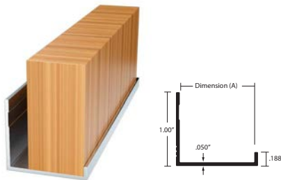
EMT-05 Millwork Flanged Angle EMT-05075 - 3/4" Depth (Dim A) EMT-05100 - 1" Depth (Dim A) EA, MF
