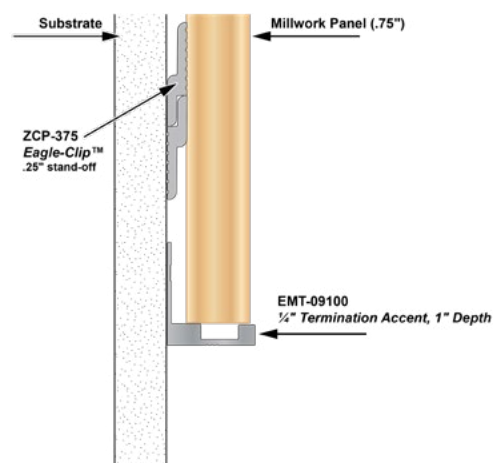
Example Installation: EMT-09100 Termination Accent with .75" Millwork Panel and ZCP-375 Eagle-Clip Z Clip Millwork Cleat.
