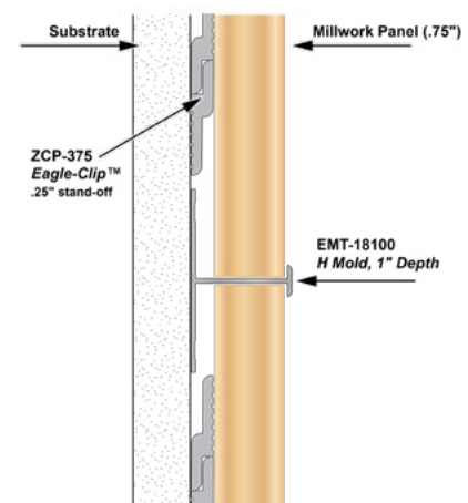
Example Installation: EMT-18100 H Mold Divider with .75" Millwork Panel and ZCP-375 Eagle-Clip Z Clip Millwork Cleat.
