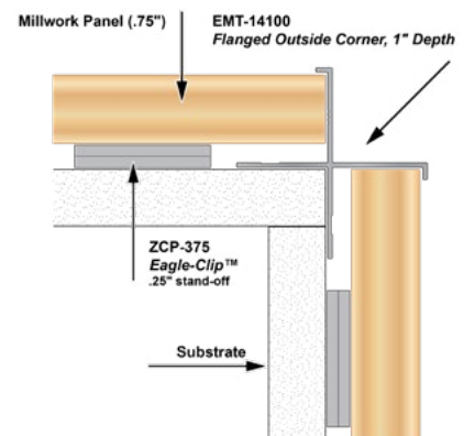
Example Installation: EMT-14100 Flanged Outside Corner with .75" Millwork Panel and ZCP-375 Eagle-Clip Z Clip Millwork Cleat.
