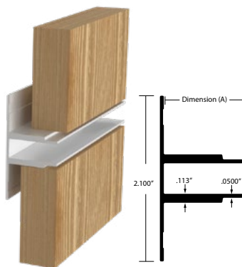
Focus Channel Reveal Close-Up Edge Detail
