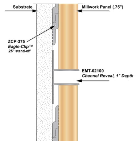
Example Installation: EMT-02100 Channel Reveal with .75" Millwork Panel and ZCP-375 Eagle-Clip Z Clip Millwork Cleat.
